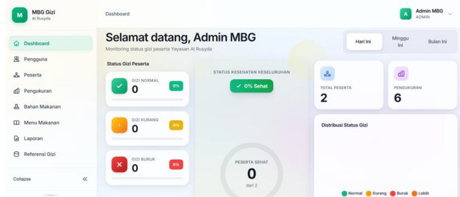
Gambar 5. Halaman Dashboard
