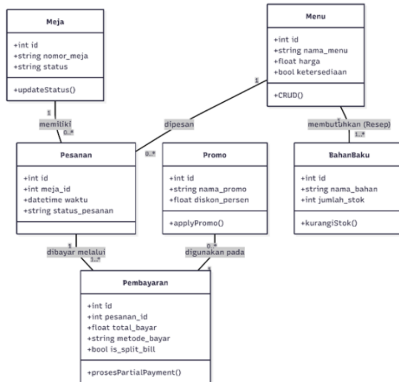
Gambar 4. Class Diagram
