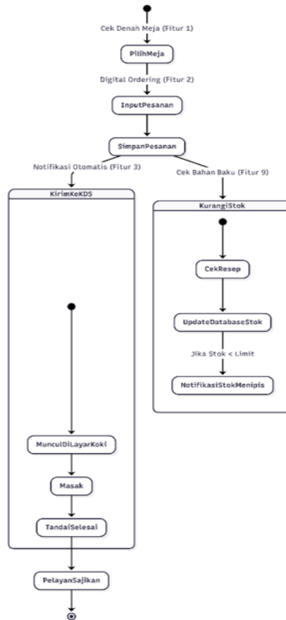
Gambar 2. Activity Diagram
