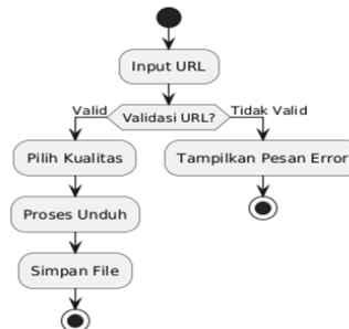
Gambar 1. Flowchart Sistem
