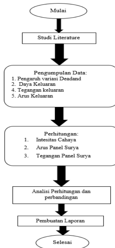
Gambar 3. Flowchart Penelitian
