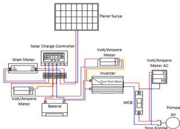
Gambar 2. Wiring Diagram Penelitian
